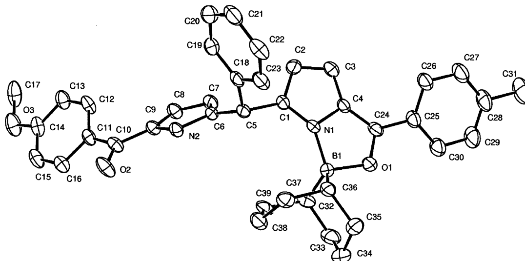
FIGURE 1. ORTEP drawing of the X-ray structure of 7b . The diacyldipyrromethane bears three distinct aryl groups and one 9-BBN unit. All ellipsoids are contoured at the 50% level. Hydrogen atoms are omitted for clarity.
